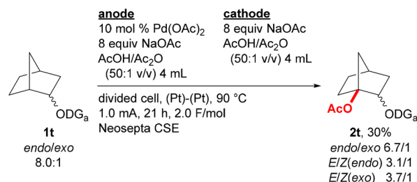
Scheme 1 Reaction of norbornan-2-ol derivative 1t .
